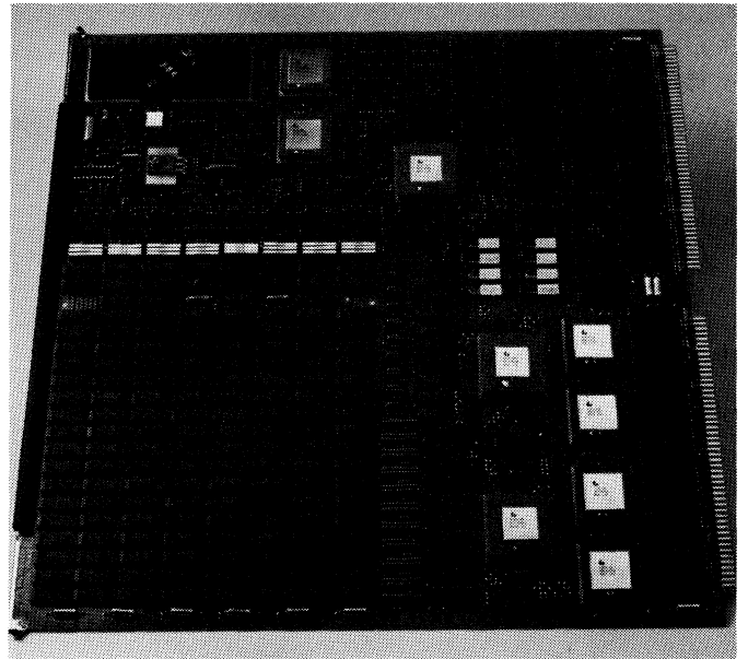
The ECLIPSE MV/8000 C uses advanced components to reduce board size, making it suitable for OEM systems integrators.
