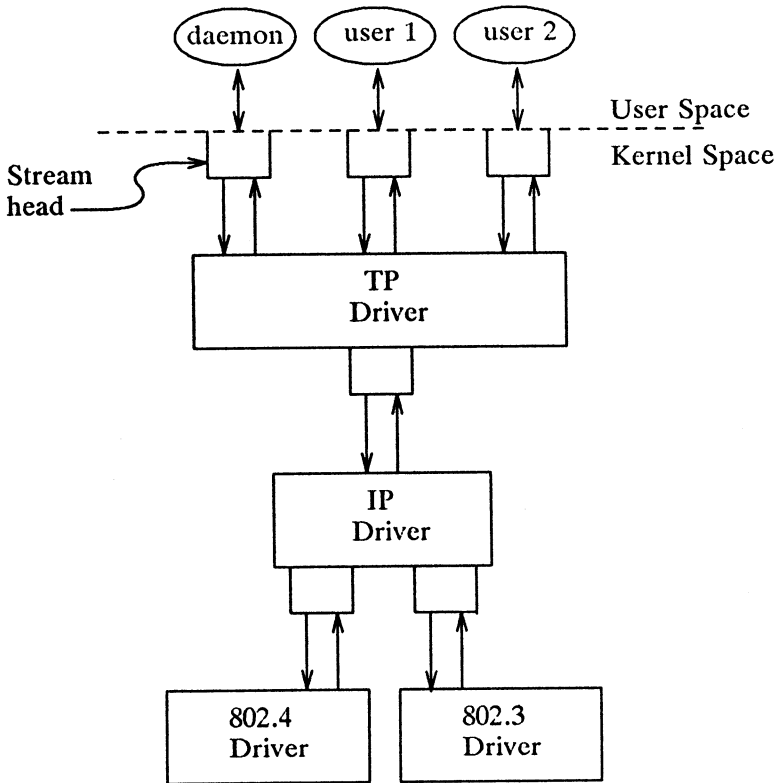
Figure 3-4: Protocol Multiplexor
