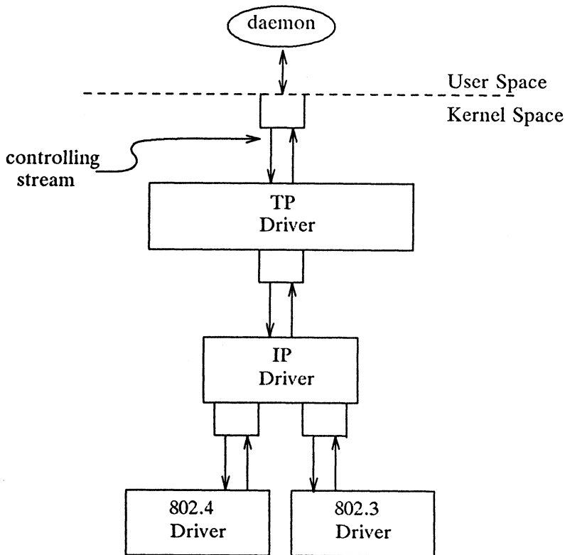
Figure 3-8: TP Multiplexor
