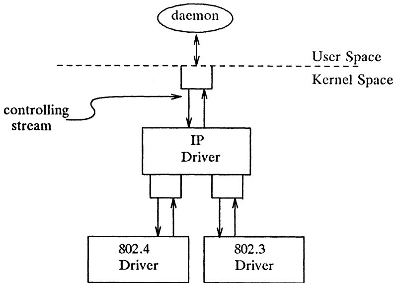
Figure 3-7: IP Multiplexor
